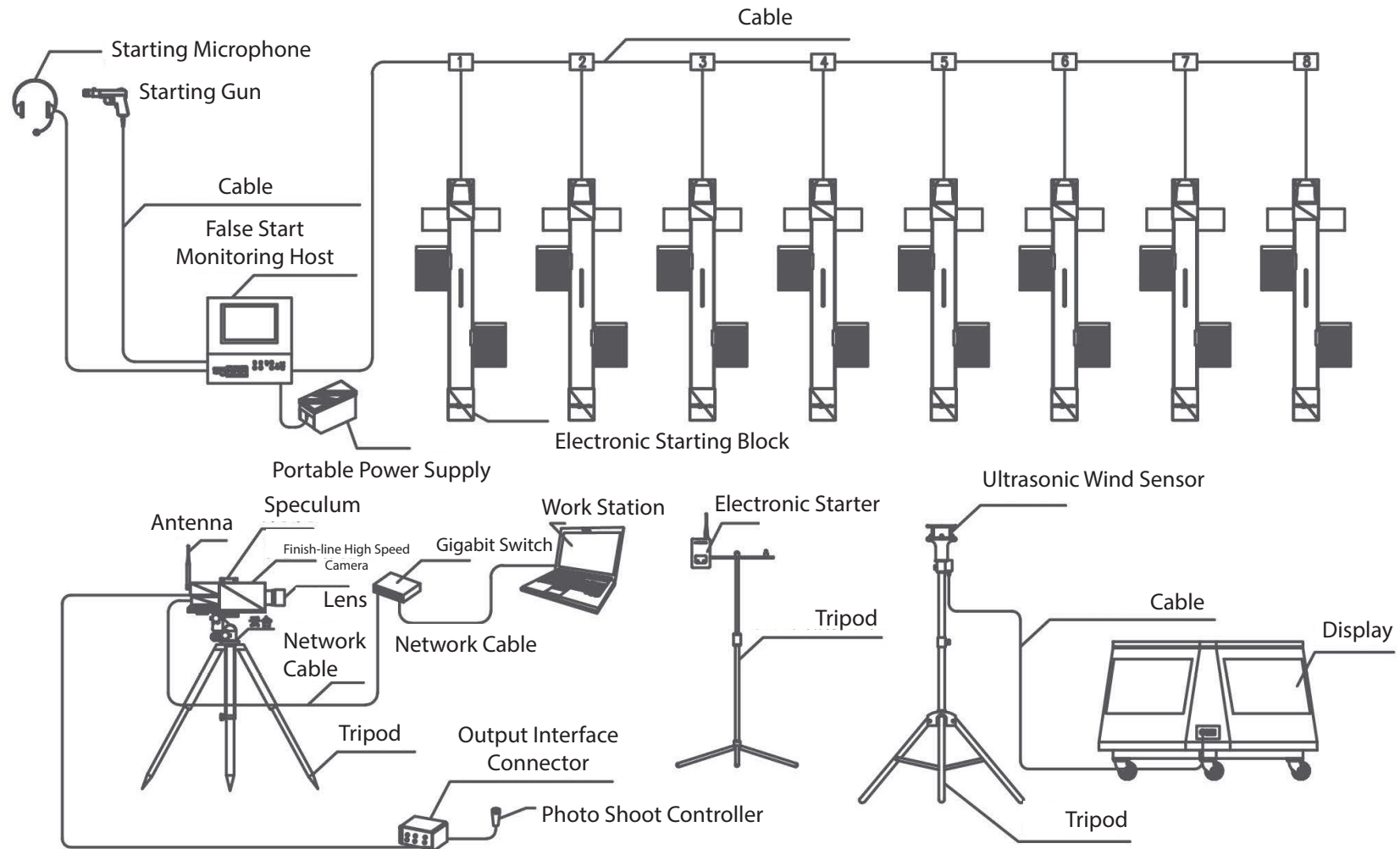
Finish-line Camera System Diagram
